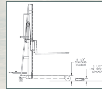
Low Profile Stacker Outtrigger Option - 2.5" Outtrigger Height
